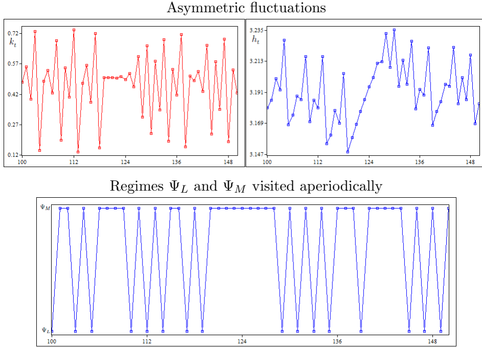
Fig. 8: \gamma = 0.05 ; Upper panel: Trajectory for physical (left) and human (right) capital after 100 transient periods. Lower panel: Visited regime ( \Psi_L, \Psi_M, \Psi_R ) of k_t .
