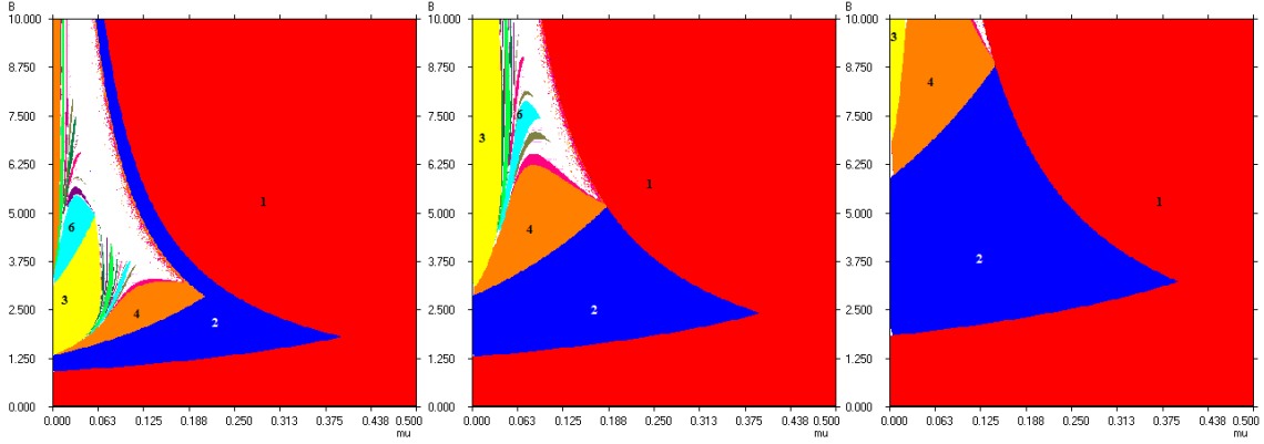
Fig. 3: (\mu, B) plane with \gamma = 0.05 (left), \gamma = 0.10 (center) and \gamma = 0.15 (right). Numbers indicate the periodicity of stable cycles. The white regions indicate a periodicity higher than 12.
