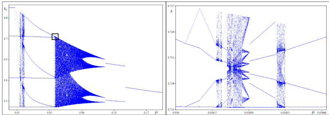
Fig. 7: Bifurcations scenario of \mu (left) and enlarged box (right).
