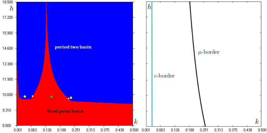
Fig. 5: Basin of attraction (left) and basin boundaries (right) with \gamma = 0.1458
