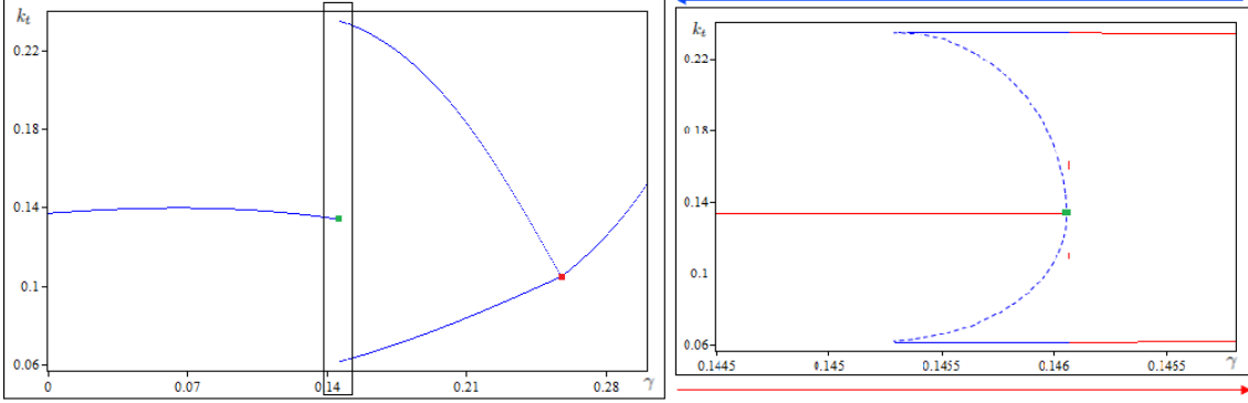
Fig. 4: Bifurcation scenario of \gamma (with B = 5, \mu = 0.25 ); arrows indicate the direction of computation
