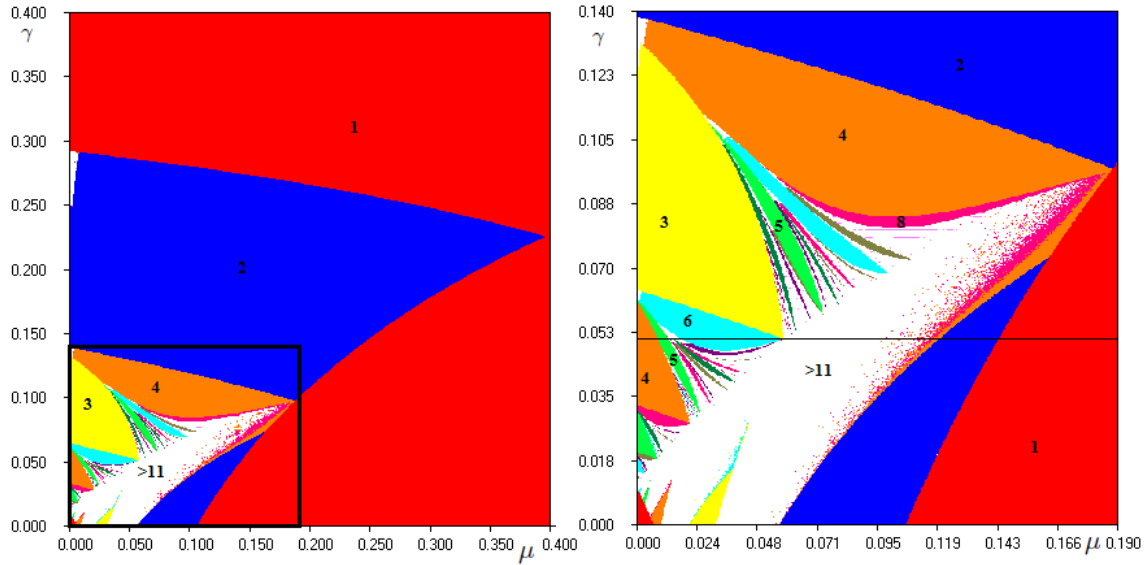
Fig. 6: (\mu, \gamma) plane with \alpha = 0.4 (left) and enlarged box (right). Numbers indicate length of stable cycle.
