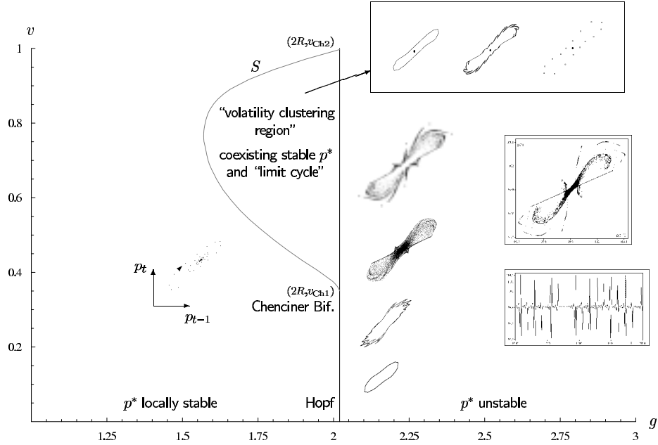
Fig. 1. Bifurcation diagram in the g - v -plane. Projections of attractors to the p_{t-1} - p_t -plane in the corresponding parameter regions are plotted. At points (2R, v_{Ch,i}) , i = 1, 2 , Chenciner bifurcations occur. These points lie on the Hopf bifurcation line g = 2R and are connected by a curve S corresponding to a saddle-node bifurcation curve of invariant circles. Parameter values: \beta = 3 , R = 1.01 , \bar{y} = 1 , \alpha = 10 , a\sigma^2 = 1 , parameter values for the attractor and corresponding price series on the right hand side, showing intermittent chaos: \beta = 20 , g = 2.1 , v = 0.5 .
