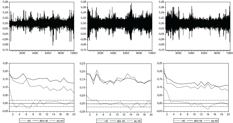
Fig. 2. Returns series (top panel) and autocorrelations of returns, absolute returns and squared returns (bottom panel) for daily S&P 500 data (08/17/1961–05/10/2000, the October 1987 crash and the two days thereafter have been excluded; left panel) and data generated by our model. Middle: performance measure minus squared prediction errors (11), right: performance measure accumulated profits (10); parameter values: \beta = 2 , R = 1.001 , v = 1 , g = 1.89 resp. 1.9, \bar{y} = 1 , p^* = 1000 , \alpha = 2000 resp. 1800, \eta = 0 resp. 0.99, a\sigma^2 = 1 , \varepsilon_t \sim N(0, 10) , \delta_t \equiv 0 .
