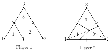
Figure 3: The best response regions of the game.
