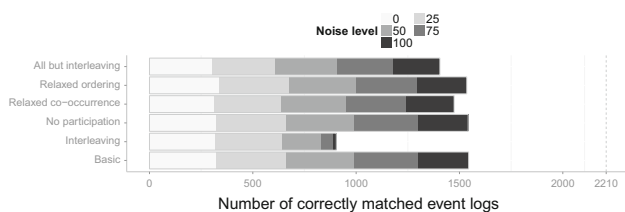
Fig. 15 DECLARE approach: number of correctly solved matchings in one-to-many setting for different noise levels
