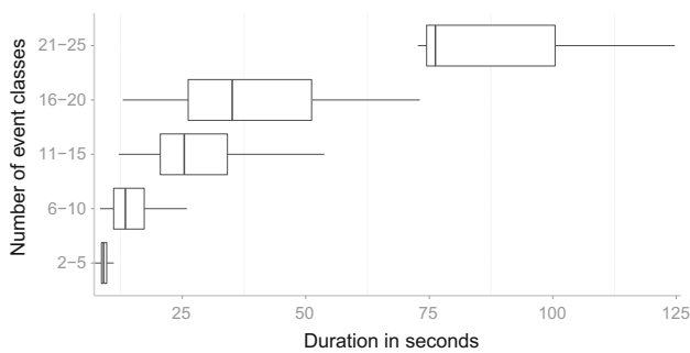
Fig. 20 DECLARE approach—basic configuration: duration of the matching depending on the number of event classes in one-to-many setting without noise (without outliers)
