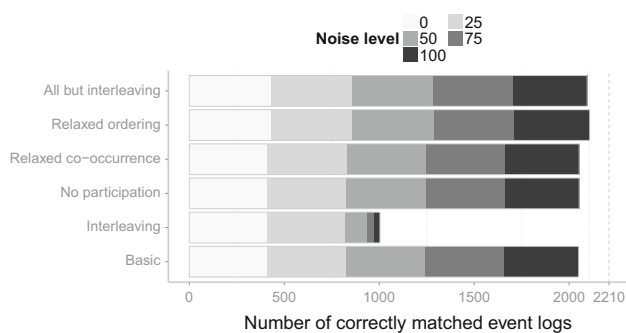
Fig. 9 DECLARE approach: number of correctly solved matchings in a one-to-one setting for different noise levels
