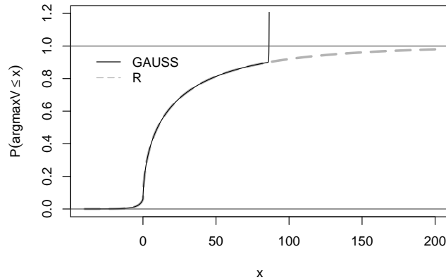
Figure 2: GAUSS vs. R for the CDF associated with the second break date, real interest data
