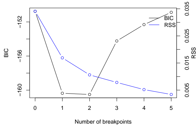
Figure 6: RSS and BIC for the Phillips curve equation.
