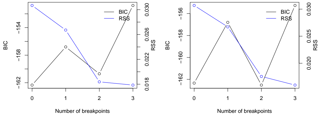
Figure 5: RSS and BIC for UK inflation data with up to m = 3 breaks for h = 8 (left) and h = 7 (right).
