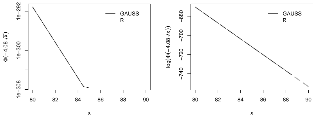
Figure 3: Computation of \Phi(-4.08\sqrt{x}) (left panel, on a log scale) and \log(\Phi(-4.08\sqrt{x})) (right panel) in GAUSS and R.
