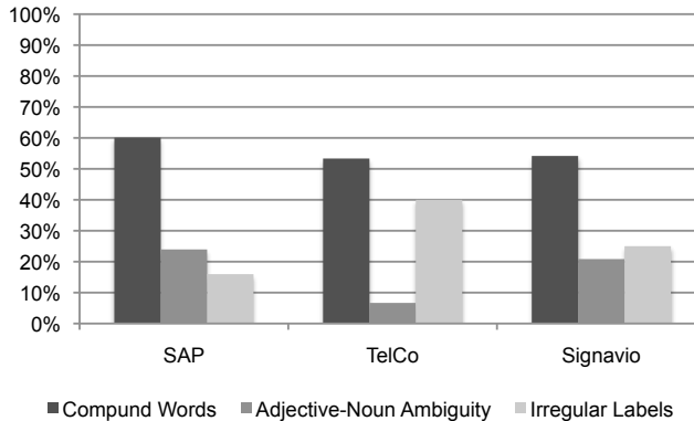
Figure 7: Distribution of Refactoring Error Sources
