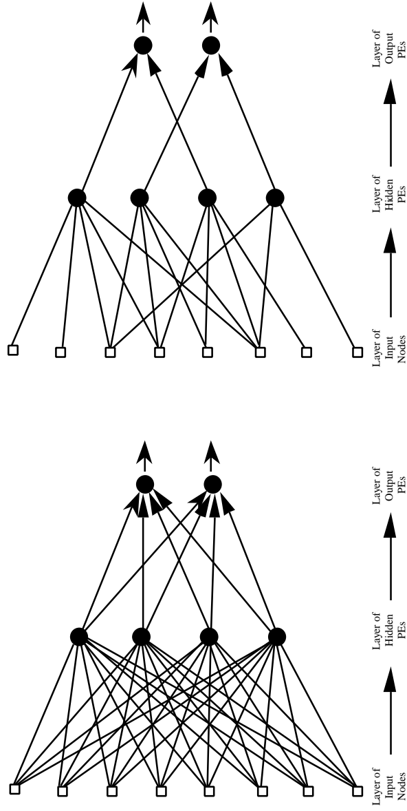
(a) Fully connected CNN
