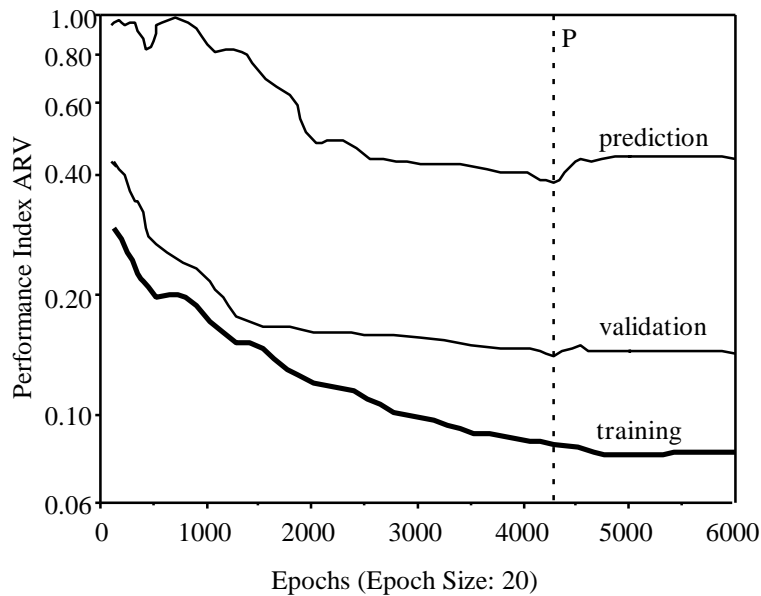
Figure 7 : Training, validation and prediction set curves of the CNN model as a function of training time in epochs (the vertical line P indicates the stopping point)
