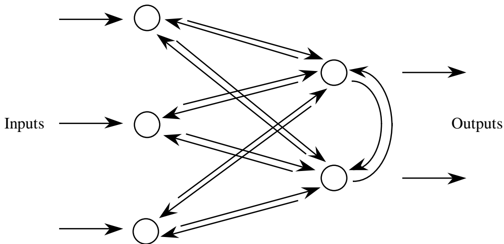
Figure 4: A recurrent computational neural network architecture
