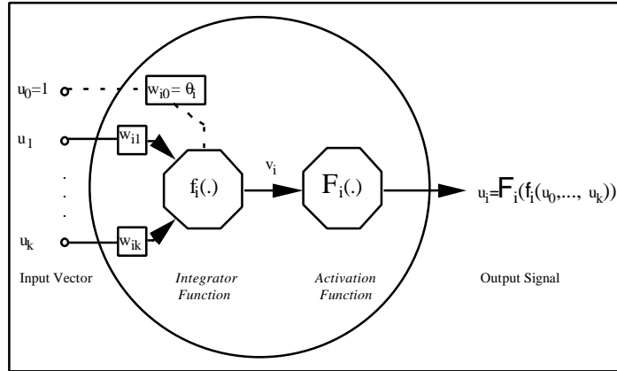
Figure 2: Generic processing element u_i
