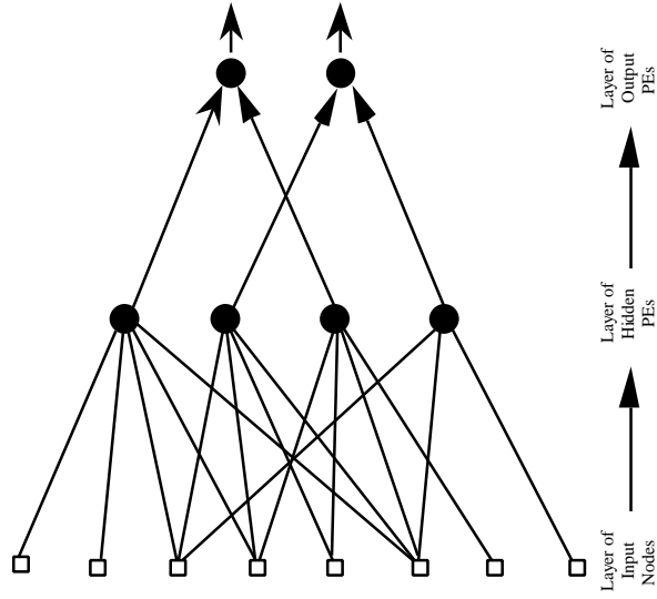
(b) Partially connected CNN
