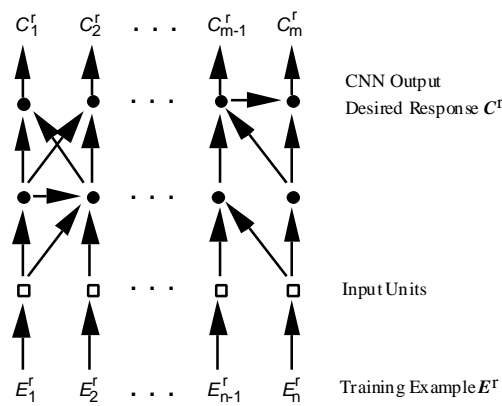
Figure 5: Training example inputs and outputs for a supervised learning model
