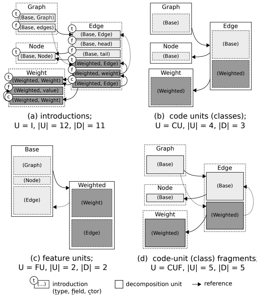
Figure 4: Dependency graphs resulting from different decompositions of GPL; U: set of decomposition units in graph; D: set of dependencies; CU: set of code units (classes); CUF: set of code-unit (class) fragments; FU: set of feature units (feature modules).
