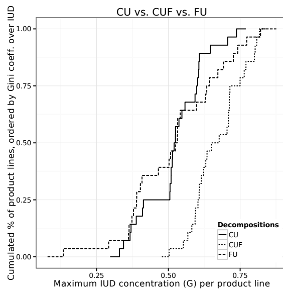
Figure 13: Three cumulative distribution curves (CDF), each representing one decomposition (CU: solid curve, CUF: dotted curve, FU: dashed curve). Each distribution curve relates a cumulated share of the 28 product lines (per decomposition, ordered by increasing IUD concentration) and a maximum IUD concentration value (G, Gini coeff.) observed for this subset of product lines. See Table 5, for the corresponding data set on Gini coefficients.
